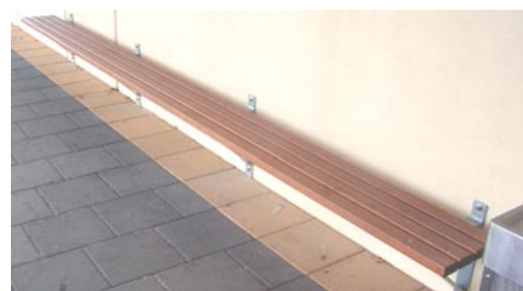
240W Wooden Wall bench 4 slat Oiled Kapur timber Galvanised steel brackets Available 2m, 3m or 4m long
