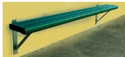
200 Aluminium Wall Bench, Natural anodised or powder coated (shown) Galvanised steel brackets Available 2m, 3m, 4m or 6m long
